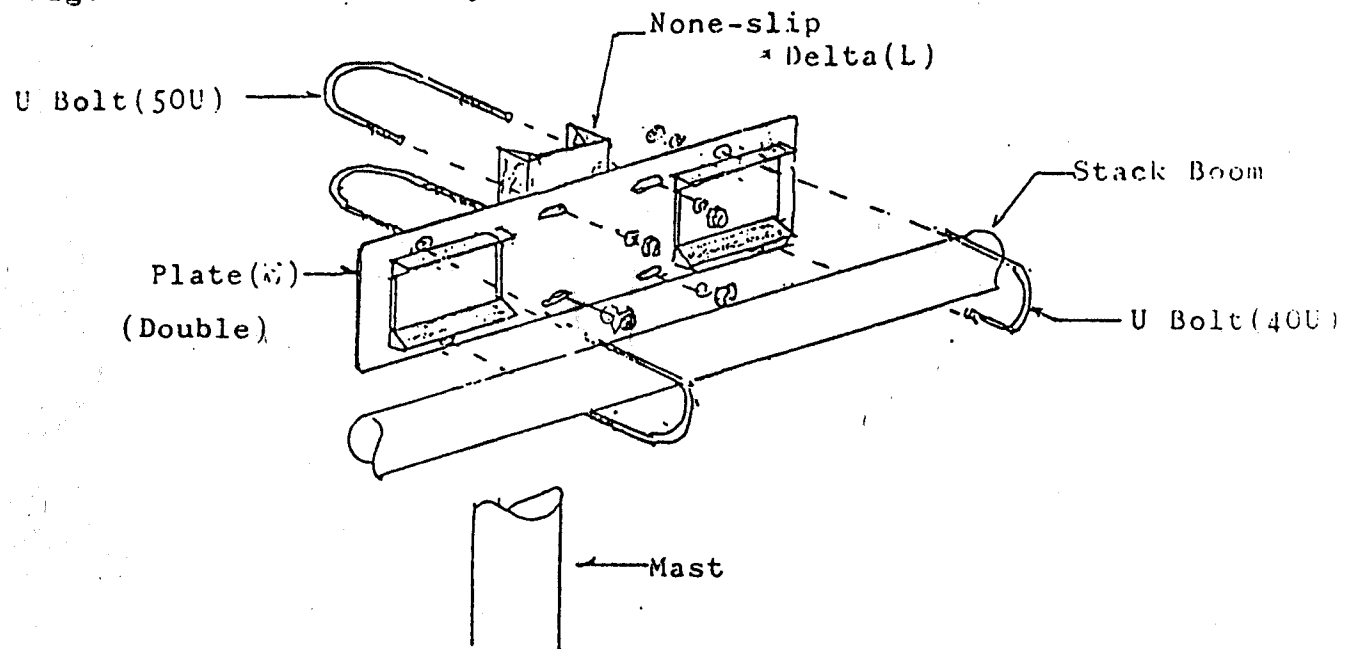
Fig.6 Cross Mount Ass'y
