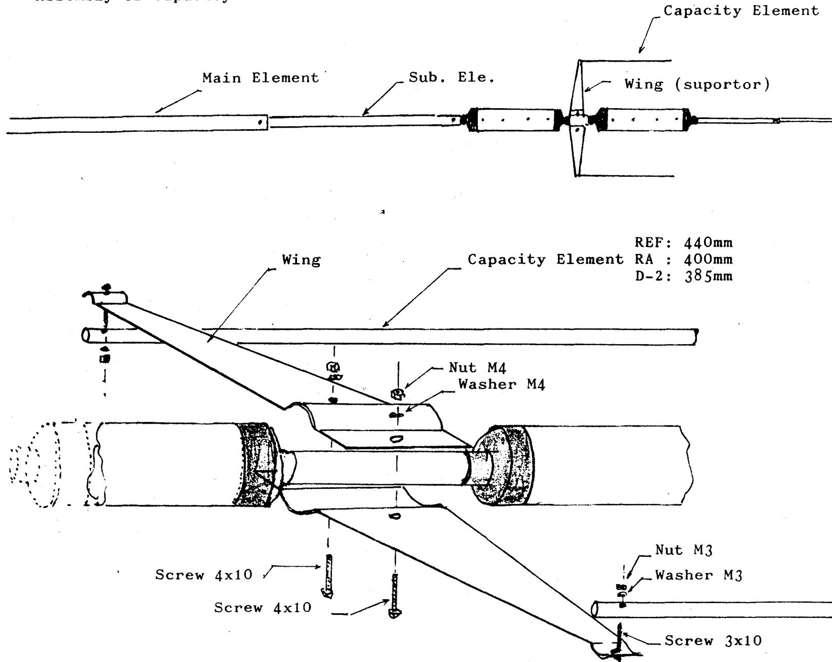
Fig. 3 Assembly of Capacity Element
