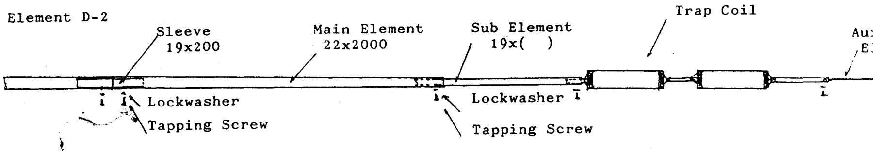
Fig.2 Assembling of Element
